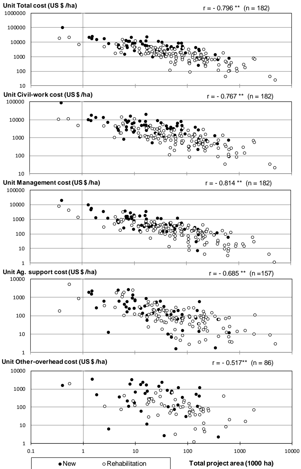
Fig. 1 Correlation between project-size (total area) and unit costs
